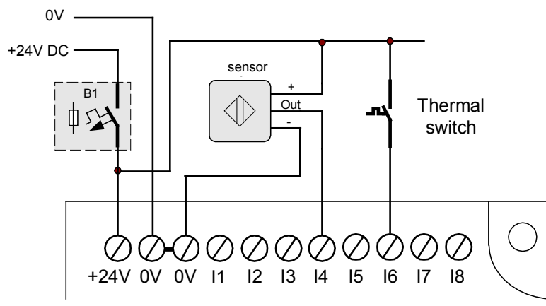
Fig 3.6.2. Input connection – proximity sensor, thermal switch contact.
