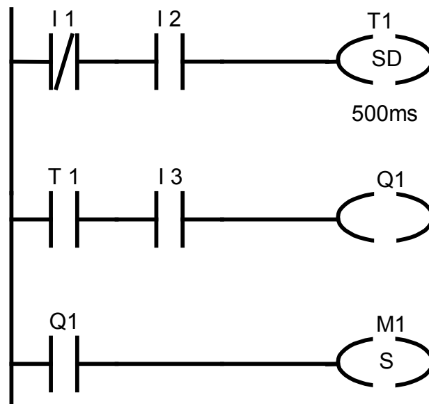
Fig. 5.2.11. Sample LAD program.
