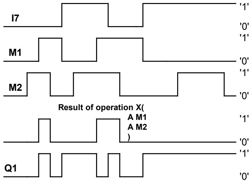
Fig. 5.1.2.10. Sample time series at I7, M1 and M2 inputs and Q1 output.
