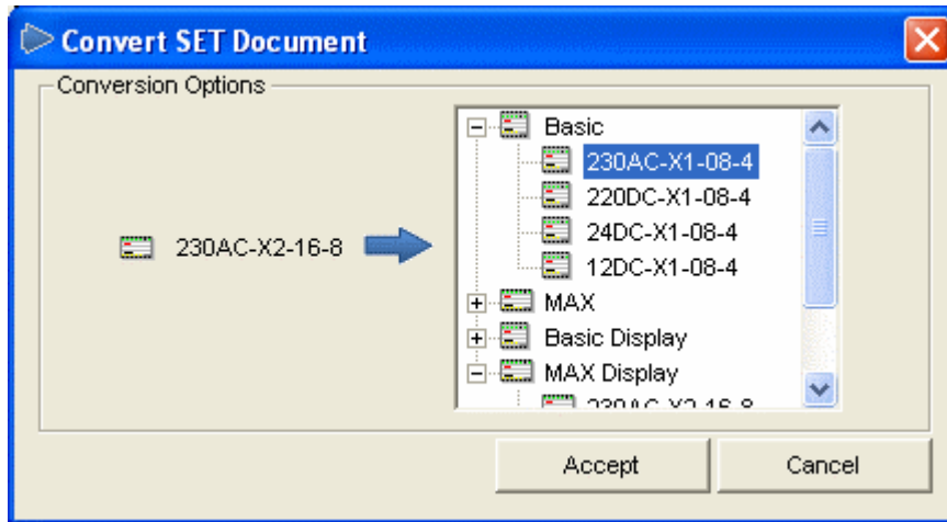
Fig. 6.15.3. Converting Settings.
