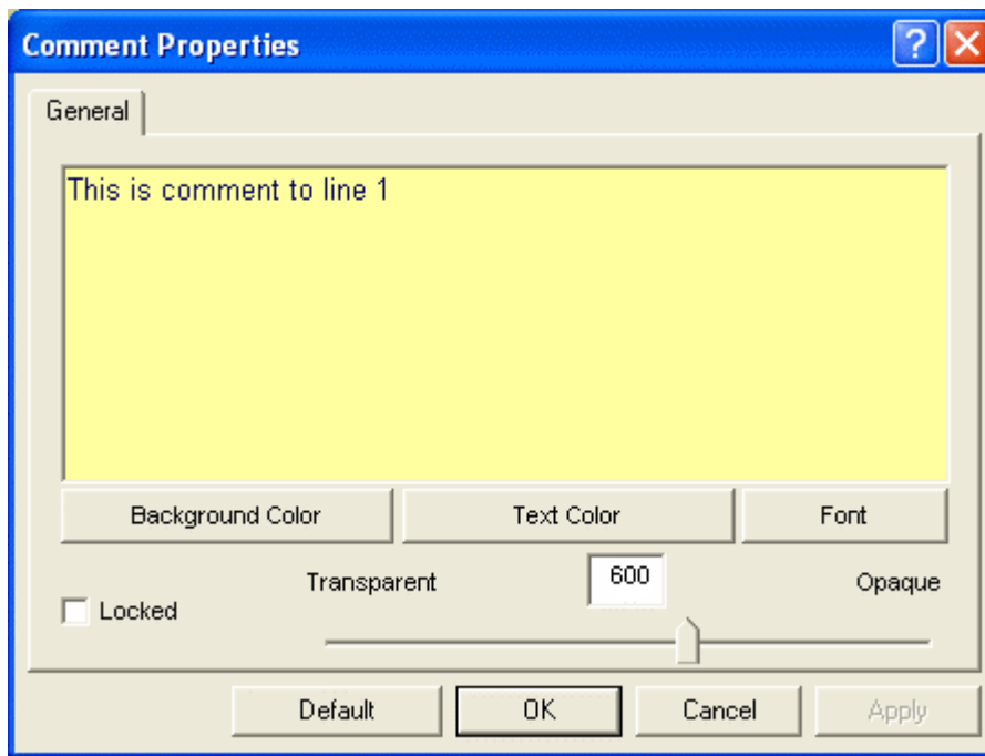
Fig. 6.8.6.3. Comment properties.
