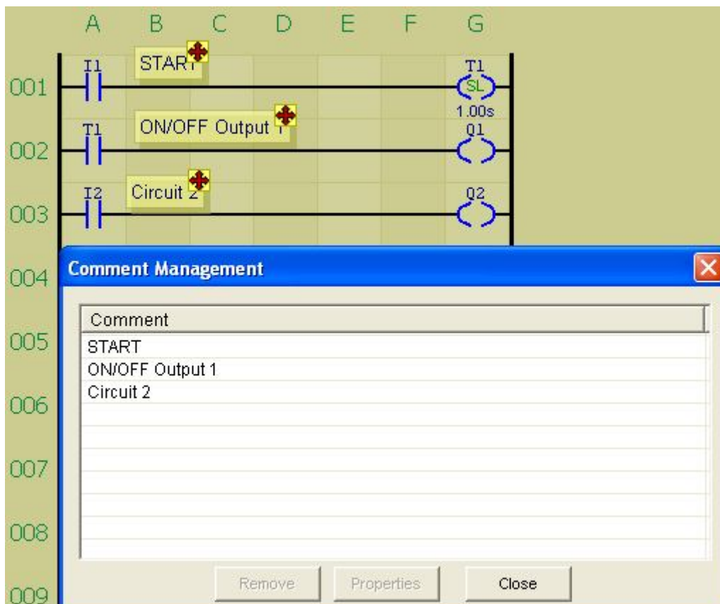
Fig. 6.8.6.4. Managing comments.
